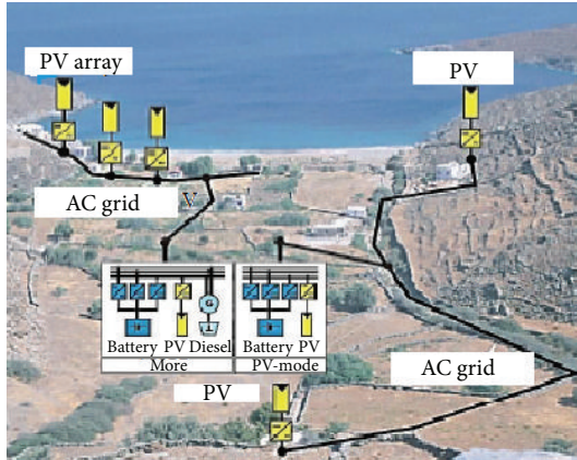
FIGURE 2: \mu G system with PV, diesel, and storage [7].
